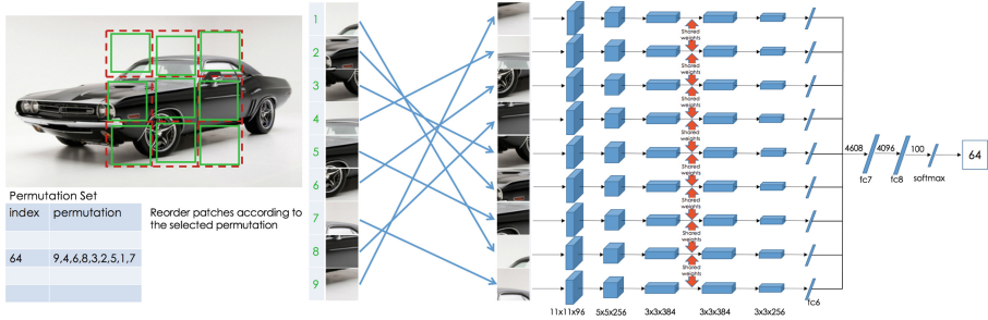
Fig. 3. Context Free Network. The figure illustrates how a puzzle is generated and solved. We randomly crop a 225 \times 225 pixel window from image (red dashed box), divide it into a 3 \times 3 grid, and randomly pick a 64 \times 64 pixel tiles from each 75 \times 75 pixel cell. These 9 tiles are reordered via a randomly chosen permutation from a predefined permutation set and are then fed to the CFN. The task is to predict the index of the chosen permutation (technically, we define as output a probability vector with 1 at the 64-th location and 0 elsewhere). CFN is a siamese-ennead CNN. For simplicity, we do not indicate the max-pooling and ReLU layers. These shared layers are implemented exactly as in AlexNet [23]. The only difference is that we set the stride of the first layer to 2 instead of 4. (Color figure online)
